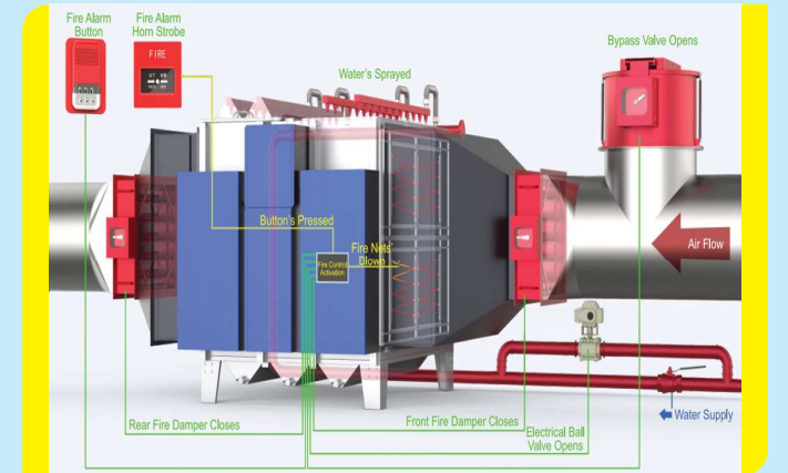
FIRE FIGHTING SYSTEM
