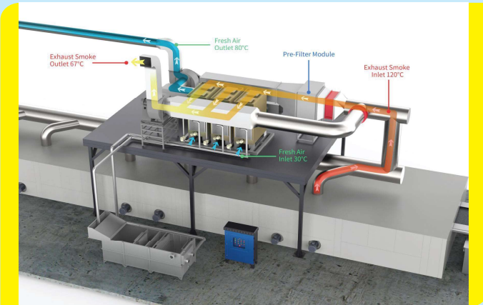
AIR TO AIR HEAT RECOVERY
