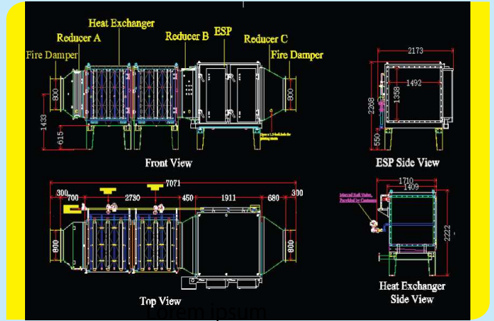
DRAWING ESP & HRU
